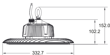
Dimension (mm)
