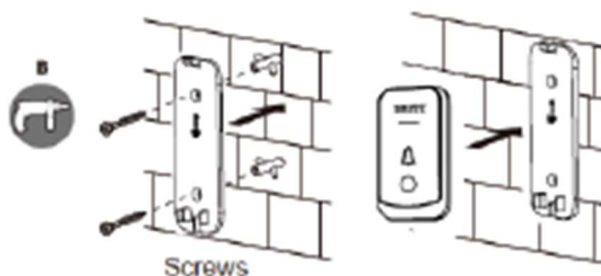
Screws
